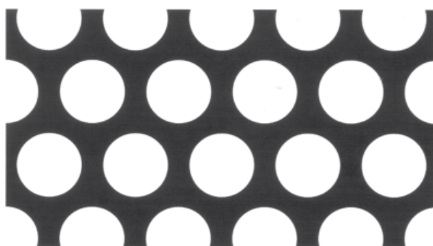
ø12,0 TD16,0 51%
